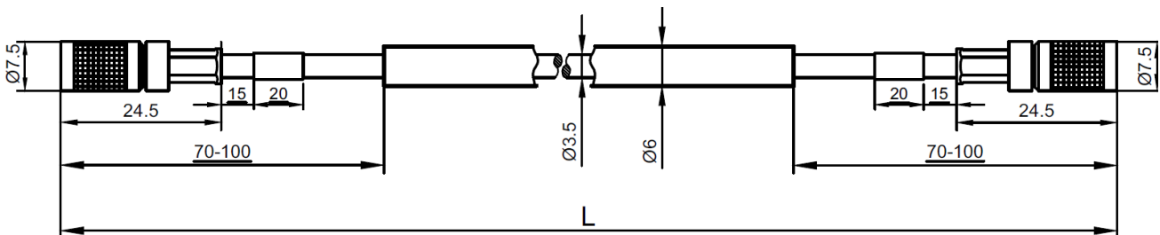
Figure 3-3) Dimensions of connection cable de82x.ec303 (PTFE tube)
