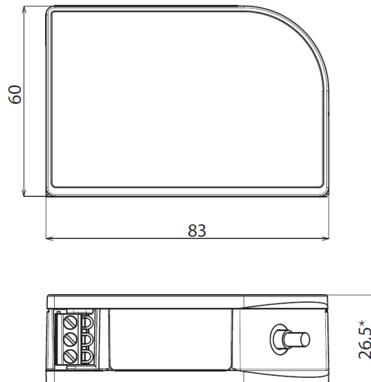
Figure 3-4 Dimensions of driver ds82x.od13Y
