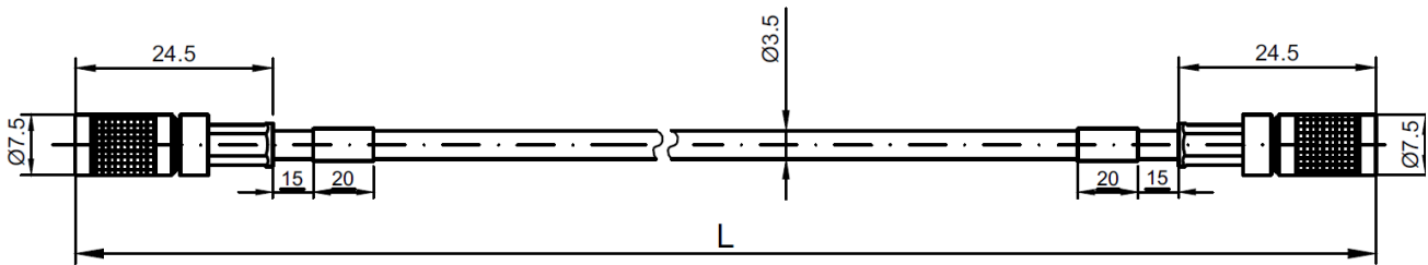
Figure 3-1) Dimensions of connection cable ds82x.ec300 (no protection)
